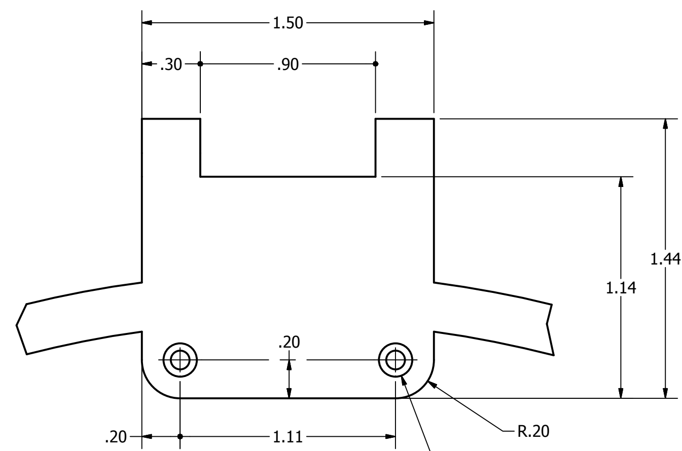
DETAIL C SCALE 2 : 1
